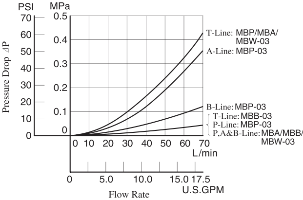
Pressure Drop
