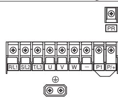
Main Circuit Terminal Assignment (B)
