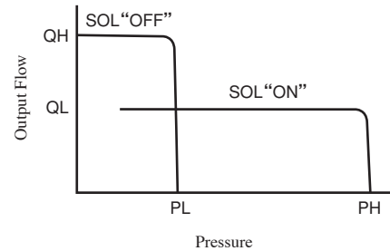
Performance Characteristics
