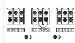
Main Circuit Terminal Assignment (B)
