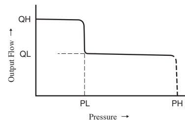
Performance Characteristics
