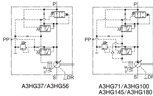
Graphic Symbols
