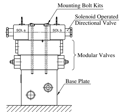
005 Series Modular Valves
